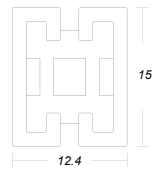
Module track light rail
